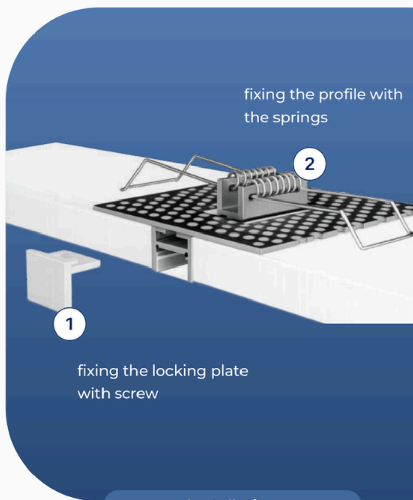
plate with springs CL-RS16/01
